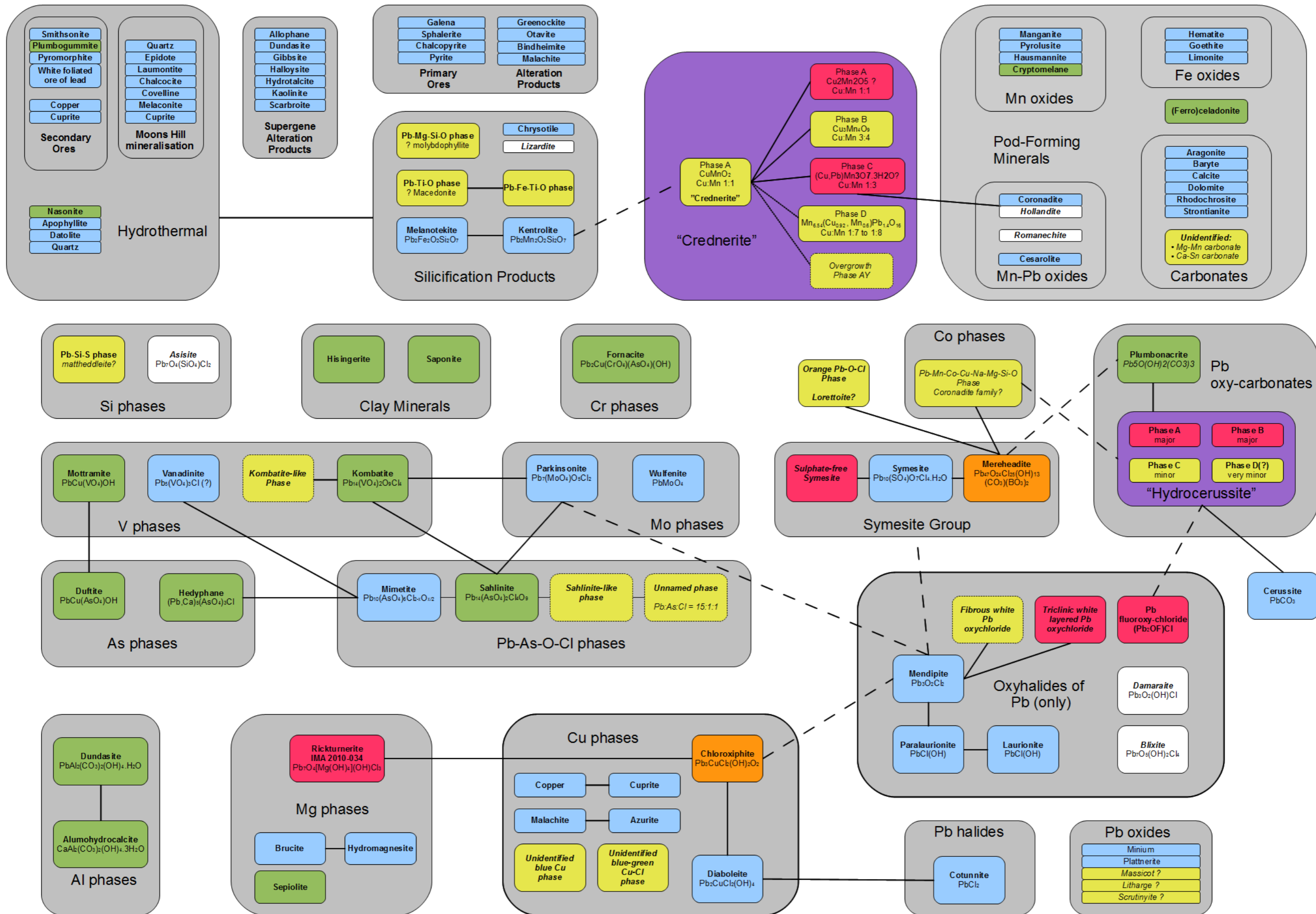
Figure 2. The 'relationship map' describing the minerals of the Mendip manganese deposits.
